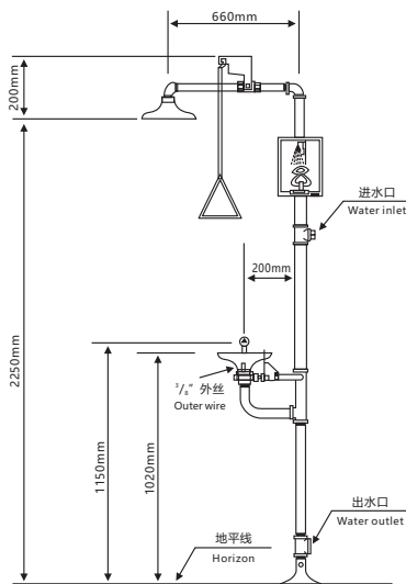
复合式洗眼器安装图 Compound eyewash installation diagram
